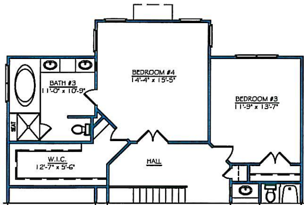
PARTIAL 2ND FLOOR OPT. BEDROOM 4
