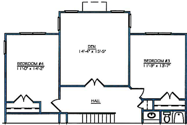
PARTIAL 2ND FLOOR OPT. DEN
